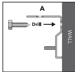
SIDE VIEW WALL MOUNT
